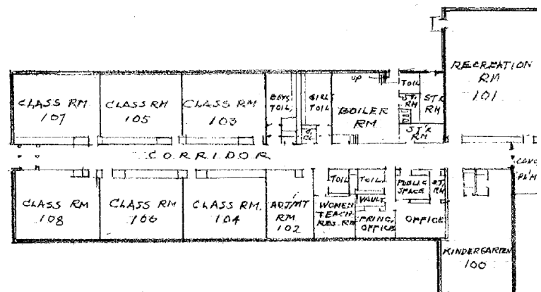
FLOOR PLAN SCALE: 1"=30'-0"
