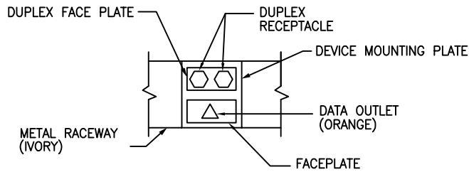
STUDENT WORKSTATION OUTLET
