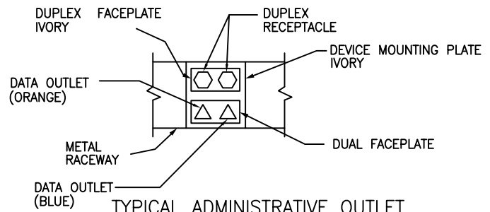
TYPICAL ADMINISTRATIVE OUTLET
