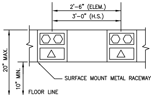
TYPICAL WORK STATION LAYOUT NOT TO SCALE
