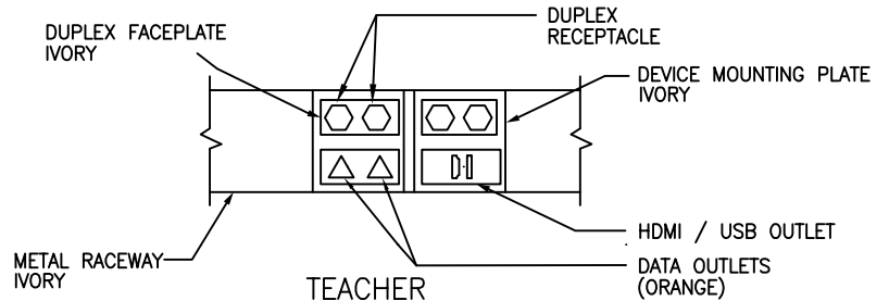
TEACHER STATION OUTLET
