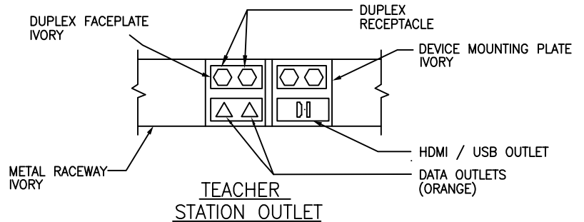
ADMINISTRATION AND FAX STATION OUTLET
