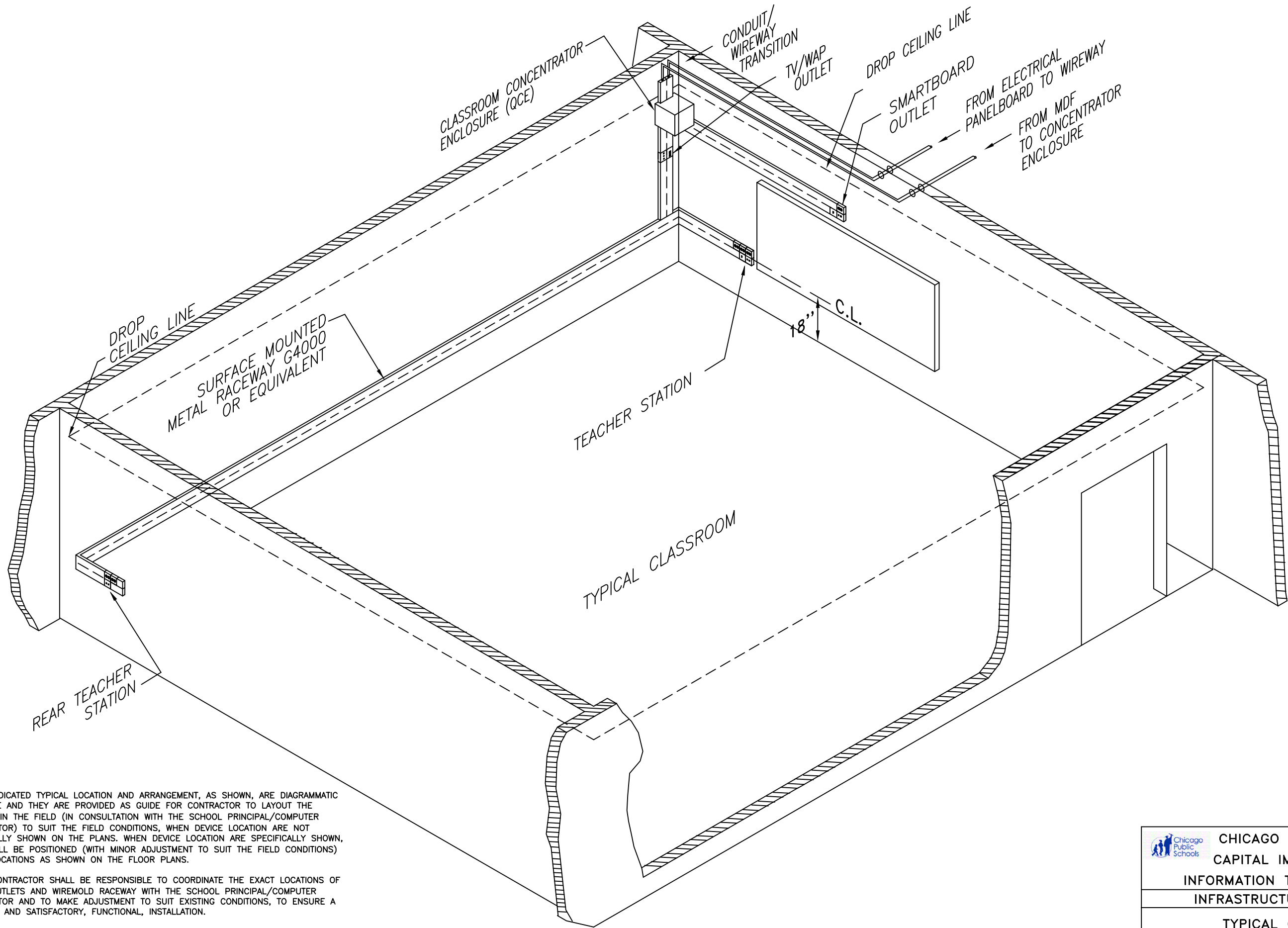
C2-8 DEVICE CLASSROOM WITH DROP CEILING NOT TO SCALE
